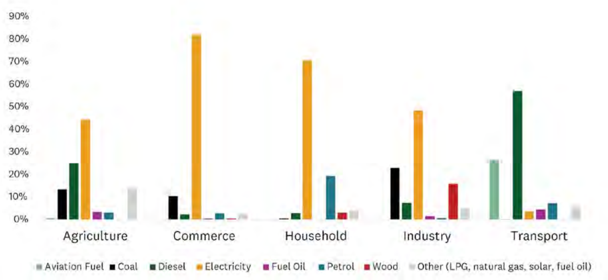
Figure 12: Estimated fuel type breakdown by sectors in Canterbury
